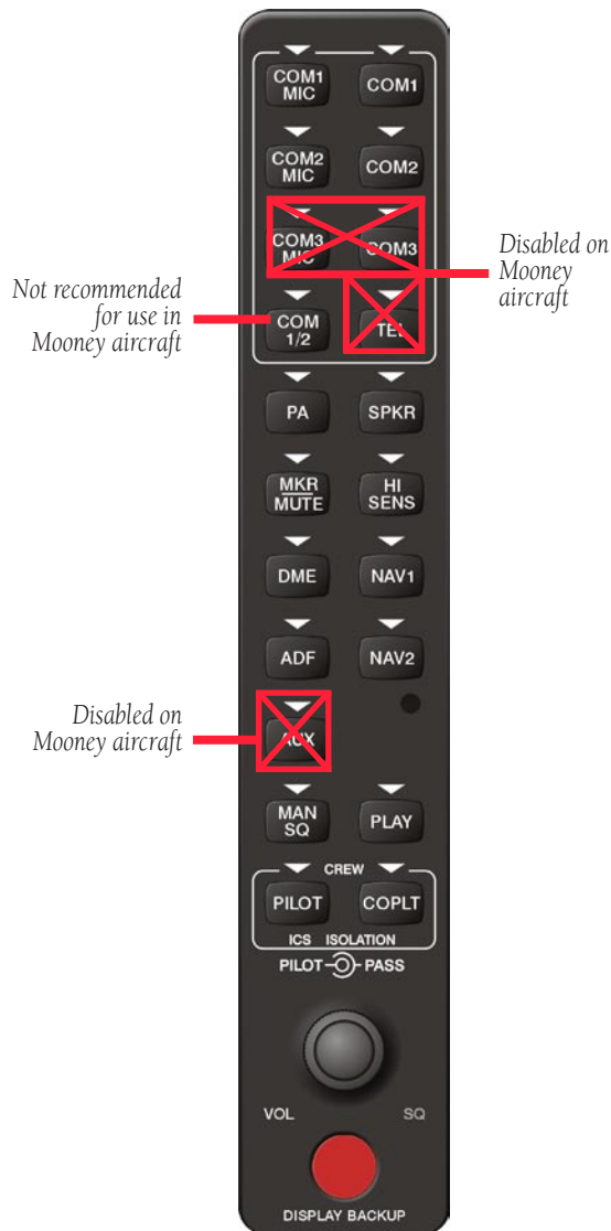
Figure 6B.1.1 G1000 Audio Panel (GMA 1347)
